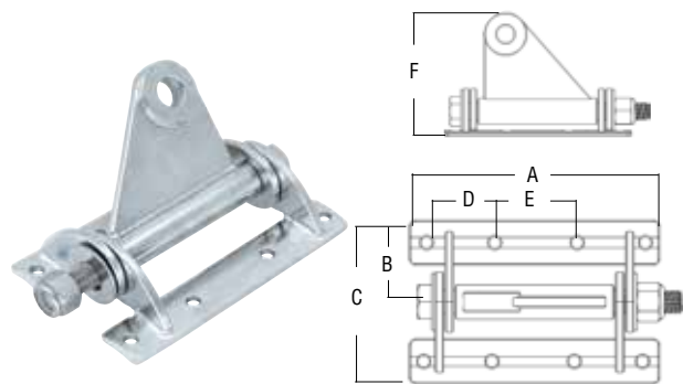
PIVOING MAST FITTINGS
