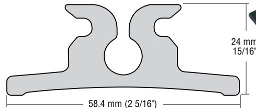
3858 Flanged track
