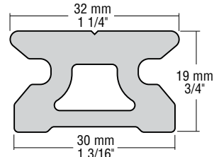
R32 Big Boat traveler track
