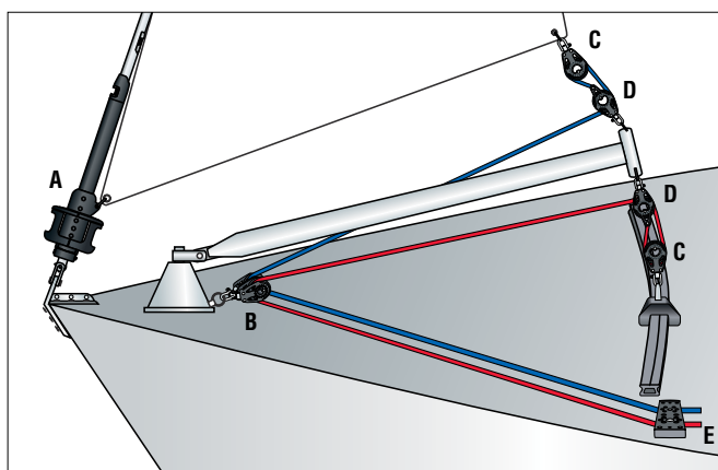
Self-tacker on Jib Boom: Self-tacking jibs and staysails work well with furling systems and jib booms. This system features two “sheets”—one controls the in and out movement of the sail much like an outhaul. The other controls the boom.
